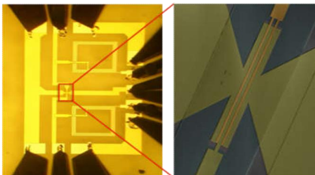
Fig.4. Graphene-based integrated circuit for wireless communications created by IBM NANOSENSORS:
